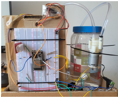
Fig. 5. Prototype hardware, view of connections on ESP32
